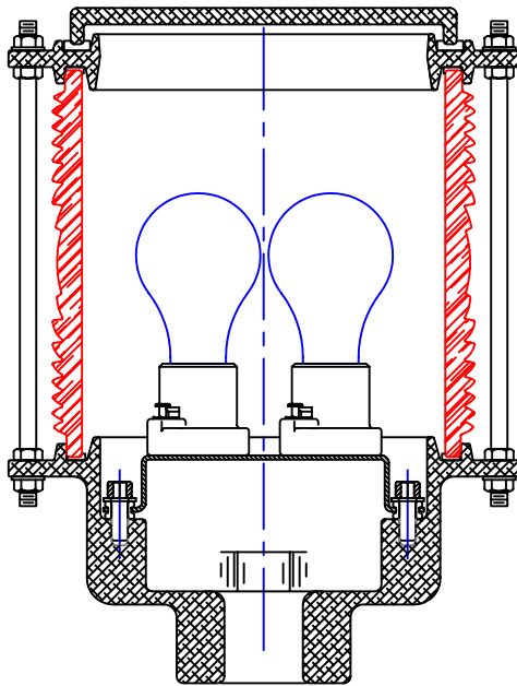
FIXTURE SECTION
